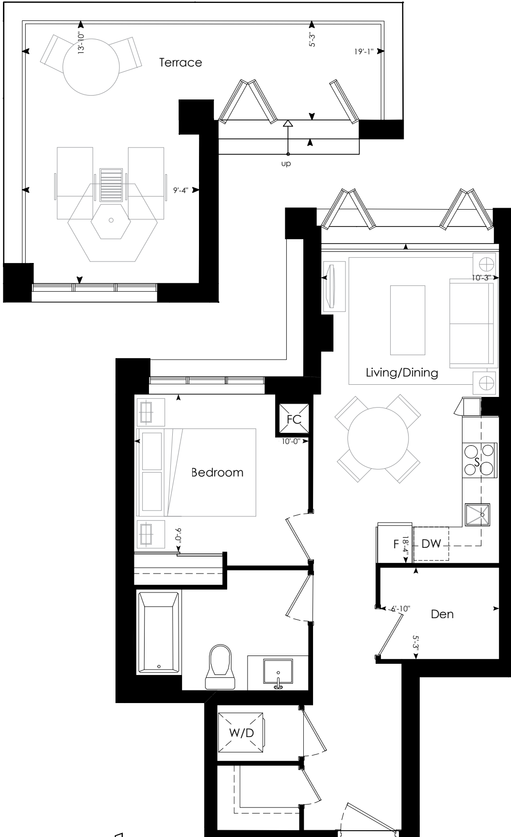
15TH-35TH FLOORPLAN
