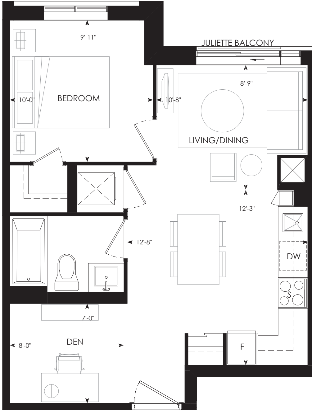
25TH-35TH FLOORPLAN
