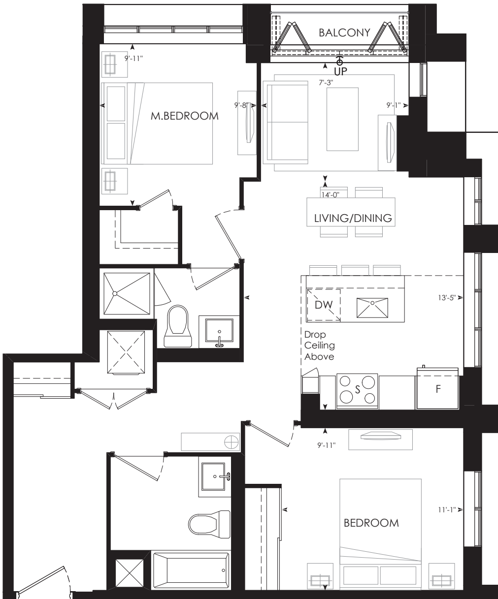
15TH-24TH FLOORPLAN
