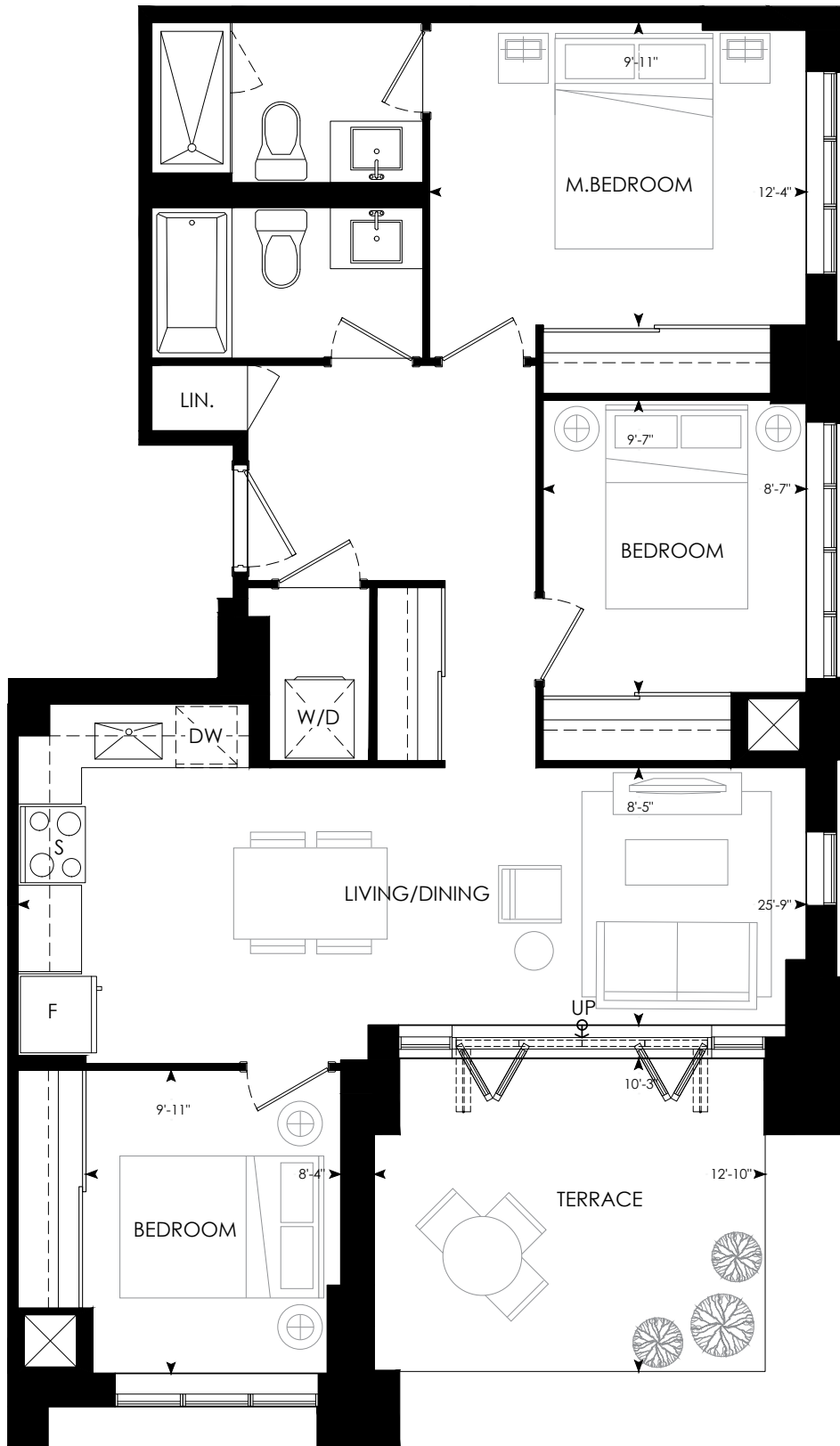
12TH FLOORPLAN
