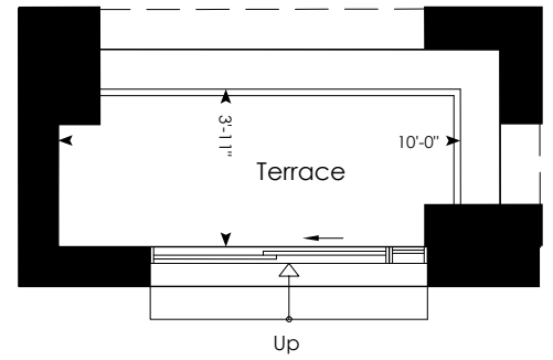
8th Floor Plan
